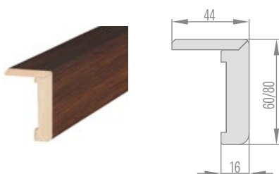
STANDARD SQUARE FOR ADJUSTABLE DOOR FRAME
